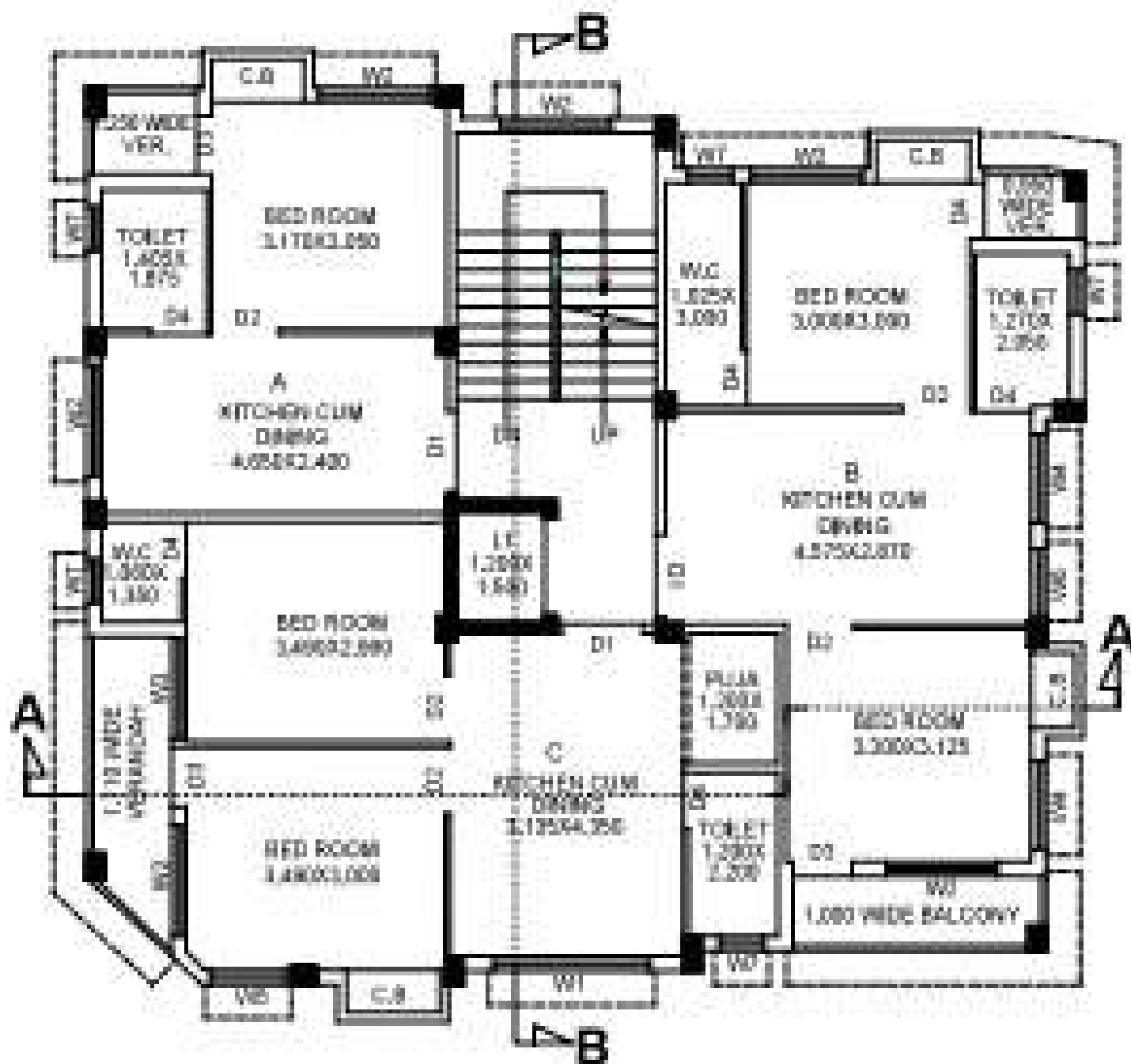
TYPICAL FLOOR PLAN (1ST TO 4TH) Scale - 1:100
